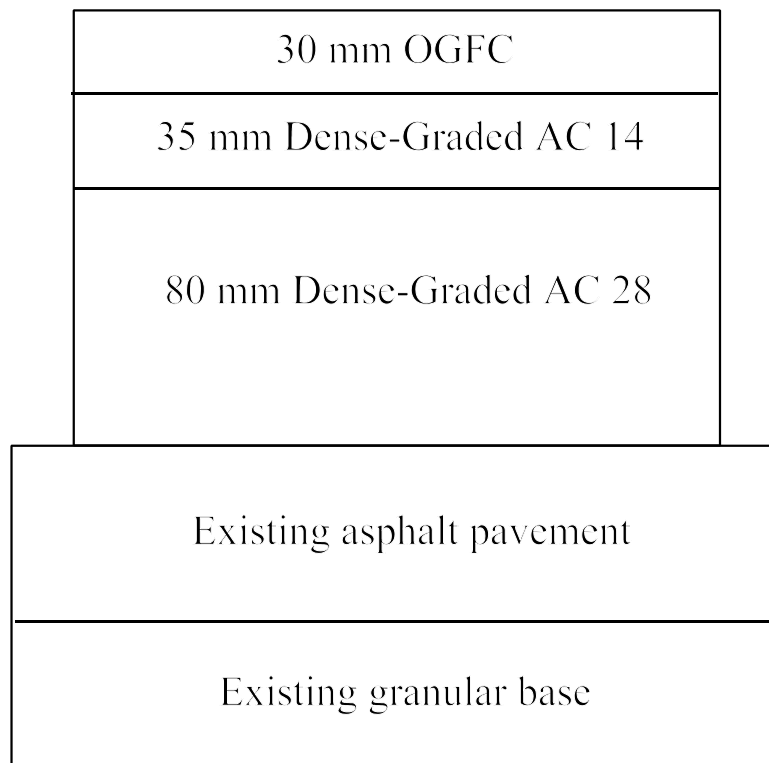
Figure 23. Courses Used in New Asphalt Overlay on Hume Highway
