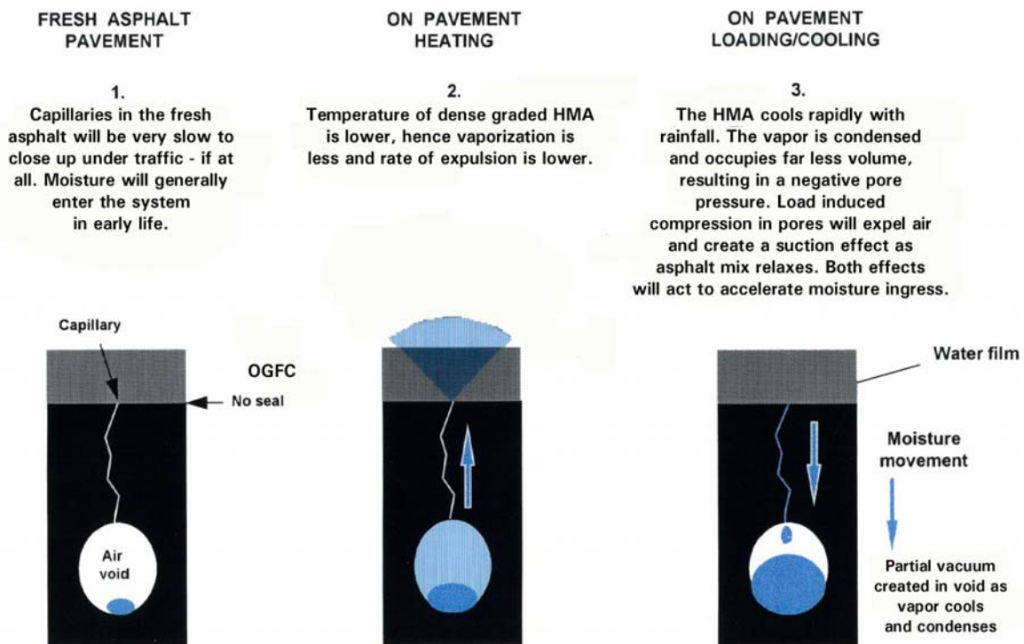
Figure 37. Schematic Representation of Moisture Movement Due to Thermal Pumping, Open Graded Friction Course (After Rickards, 4)
