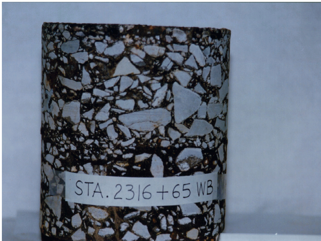
Figure 14. Pavement Core Showing an Open, Coarse-Graded F Binder Mix Underlying the OGFC (I-40)
