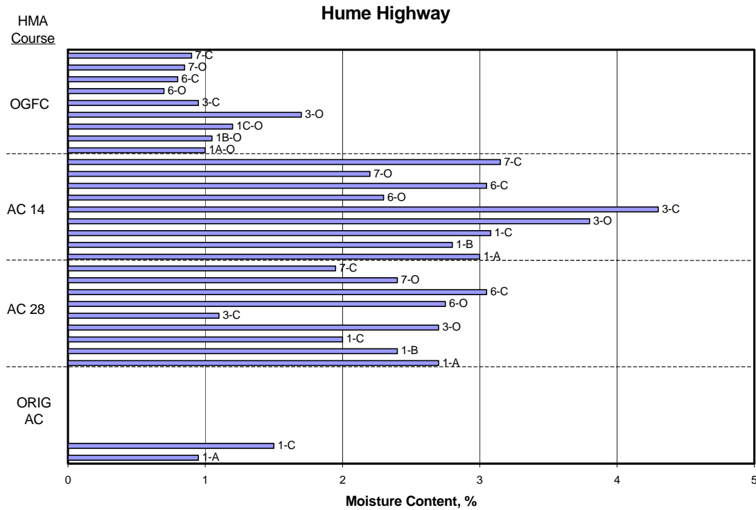
Figure 28. Moisture Content Profile at Site 1, 3, 6, and 7
