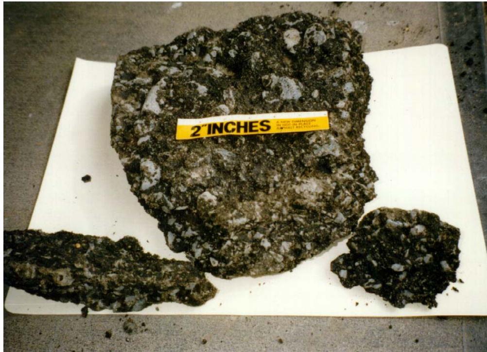
Figure 33. Badly Stripped AC 28 and AC 14 Courses
