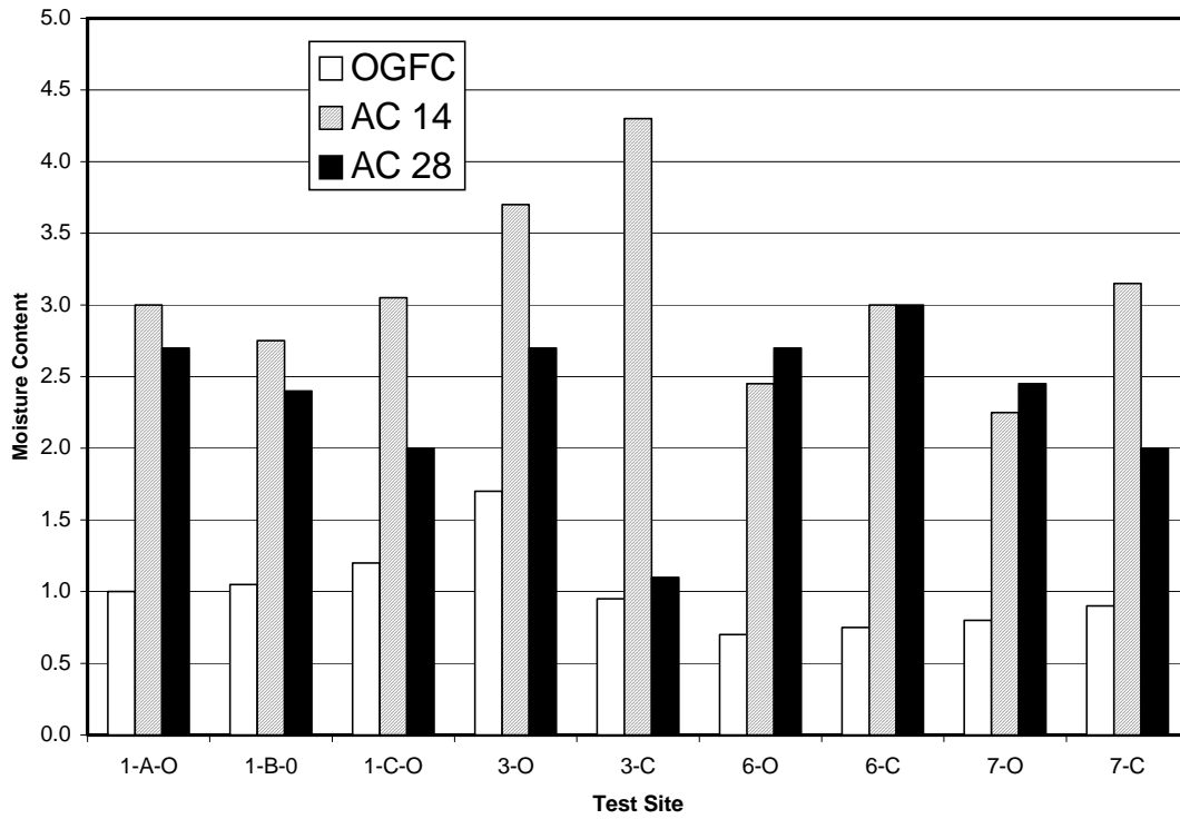
Figure 29. Comparative Moisture Contents at Sites 1, 3, 6, and 7
