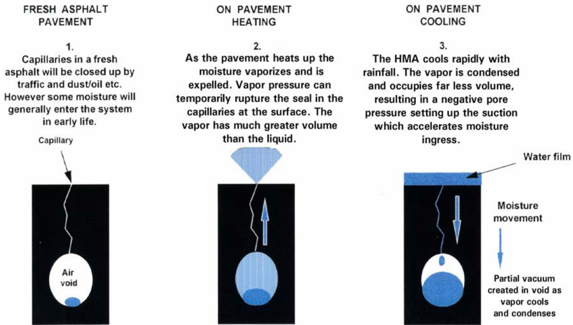
Figure 36. Schematic Representation of Moisture Movement Due to Thermal Pumping, Dense Graded Asphalt Wearing Course (After Rickards, 4)
