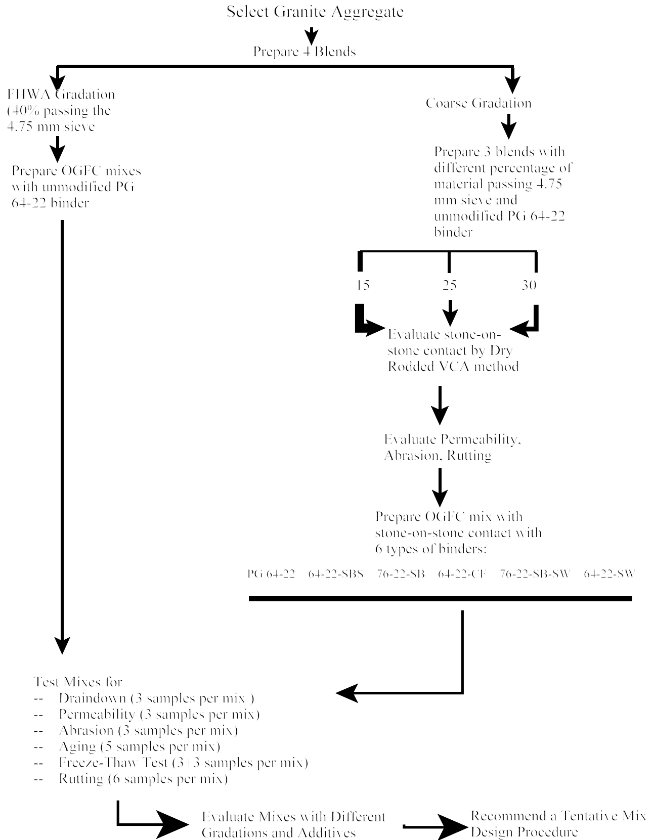
Figure 1. Test Plan
